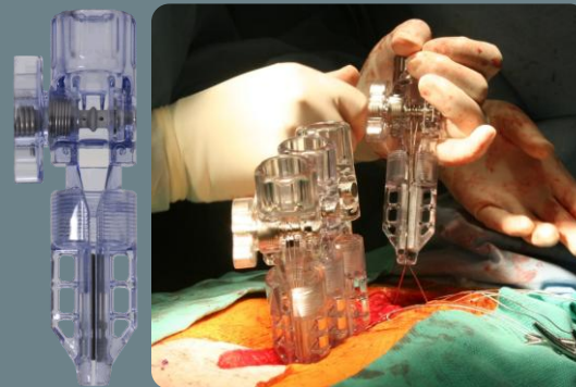
TORQ Sternum closure device
